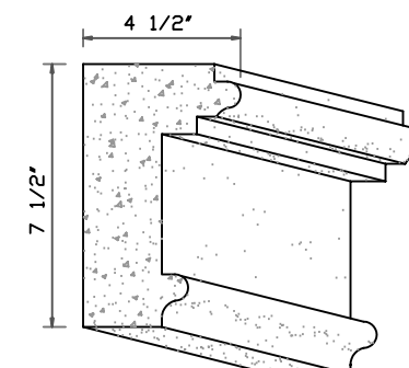
ISLEWORTH COLUMN CAPITAL TRIM
