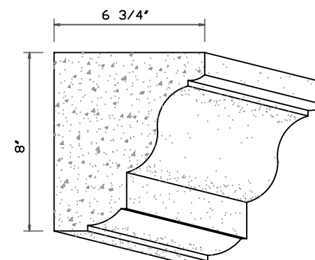
RINGLING SOFFIT TRIM
