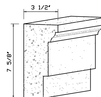
CHAMPION SURROUND TRIM
