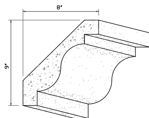
ISLEWORTH CORNICE MOLDING
