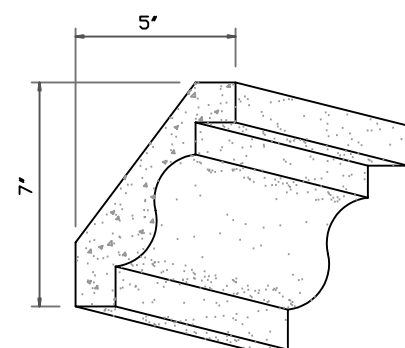
ISLEWORTH CORNICE MOLDING SMALL
