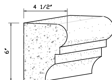
CHAMPION FASCIA TRIM
