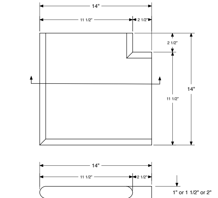
INSIDE DBL BN CORNER COPING
