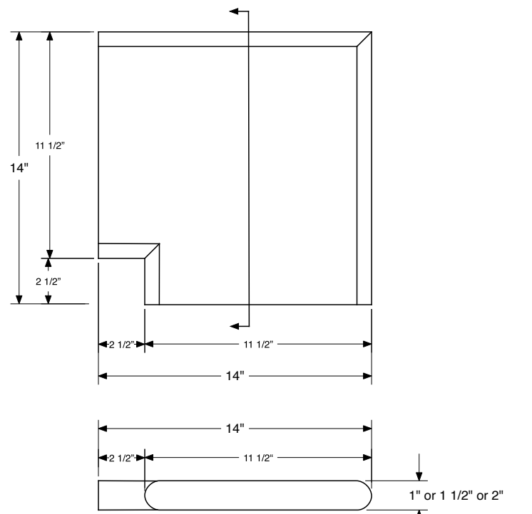
OUTSIDE DBL BN CORNER COPING
