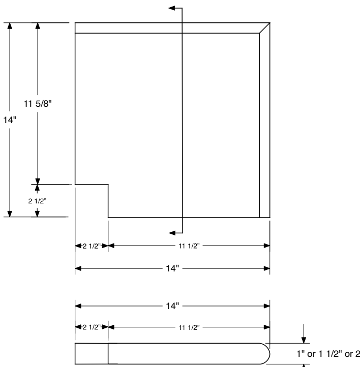
OUTSIDE SINGLE BN CORNER COPING
