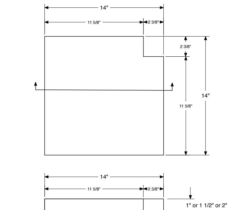
INSIDE SQUARE EDGE CORNER COPING
