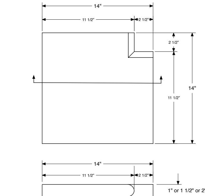
INSIDE SINGLE BN CORNER COPING
