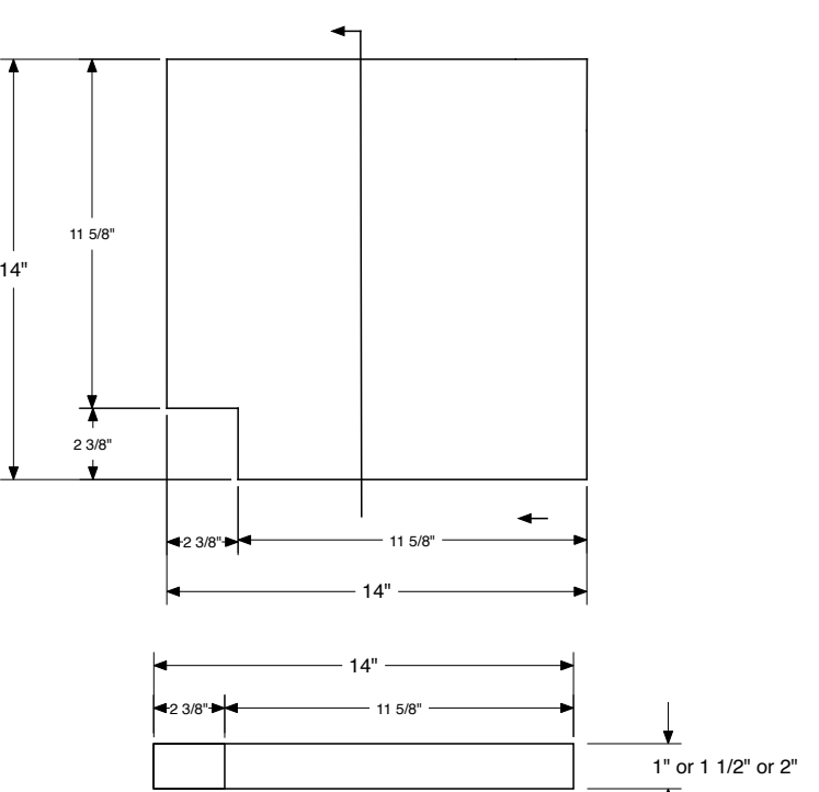
INSIDE SQUARE EDGE CORNER COPING
