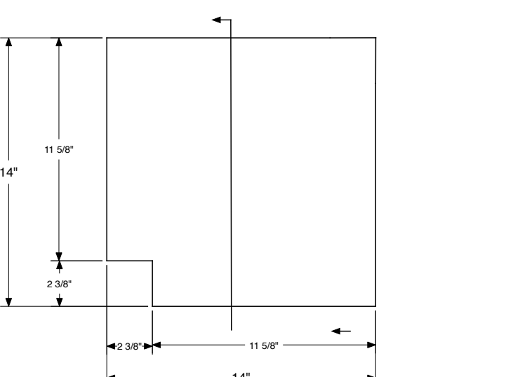
INSIDE SQUARE EDGE CORNER COPING
