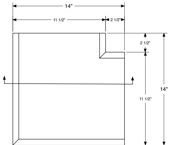
DOUBLE BN COPING
