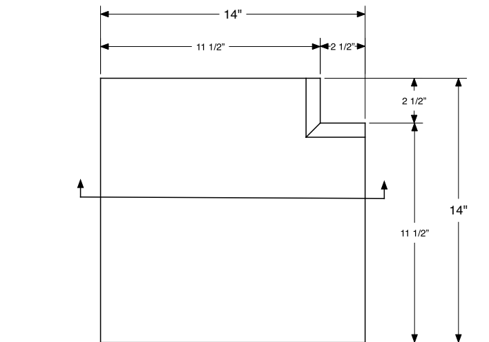
SINGLE BN COPING
